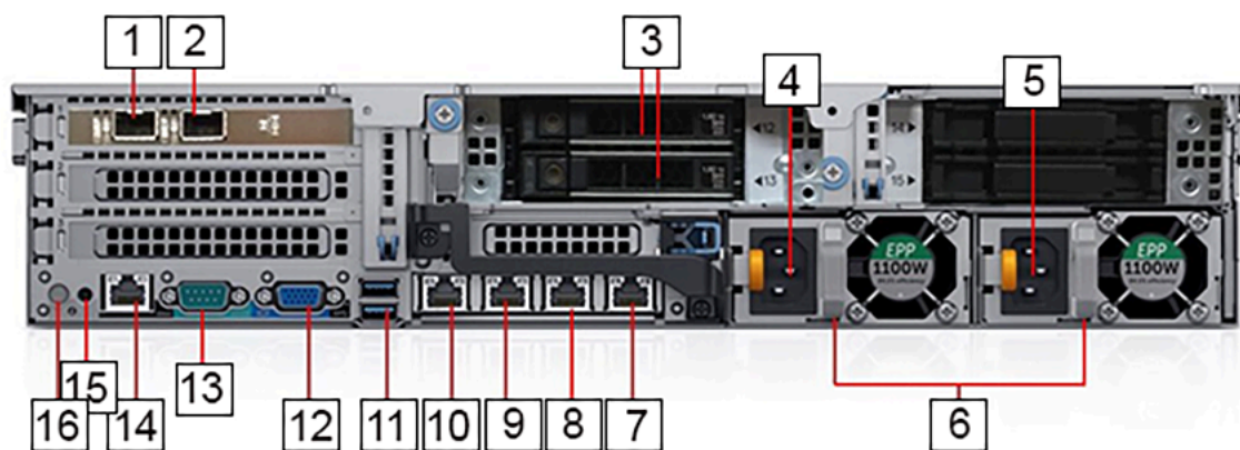
Figure 4-3: DMF Recorder Node (DCA-DM-RA3) Rear Panel
