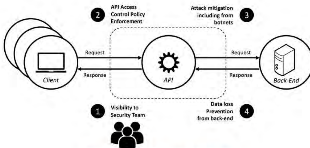
Figure 3. API Security Methods
